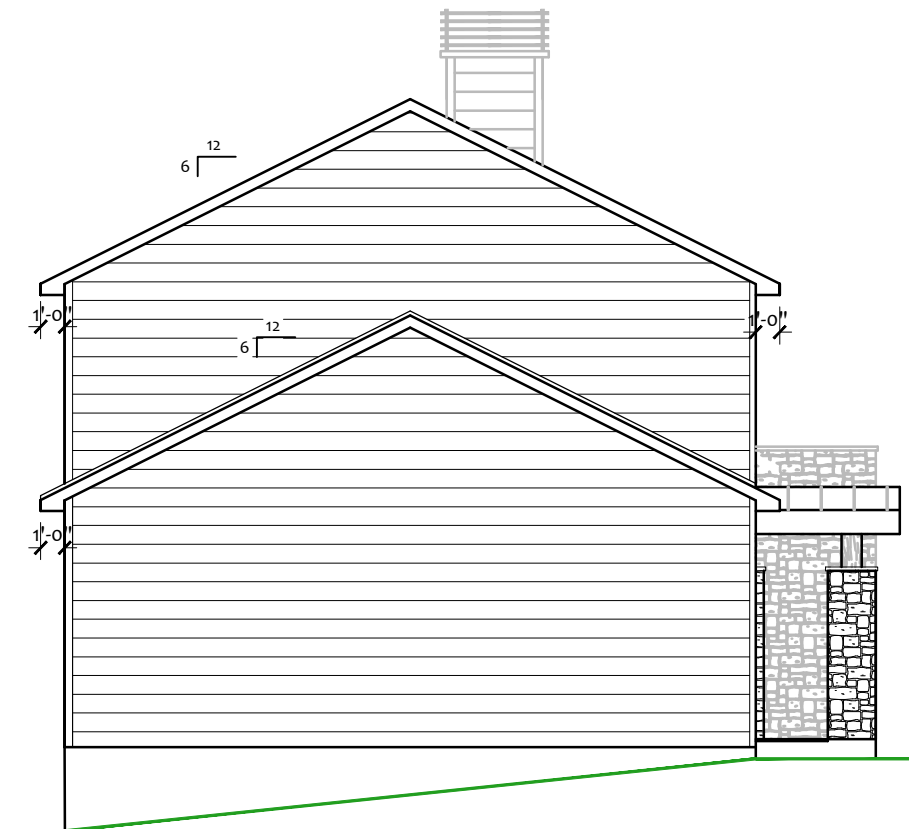
EAST ELEVATION
