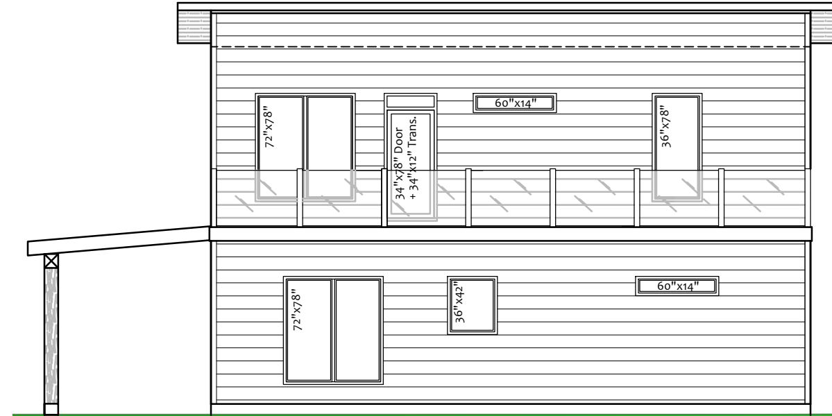
SIDE ELEVATION
