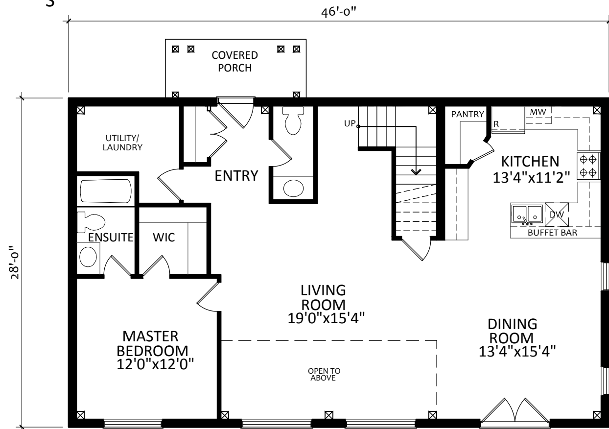
GROUND FLOOR PLAN 1288 sq.ft.
