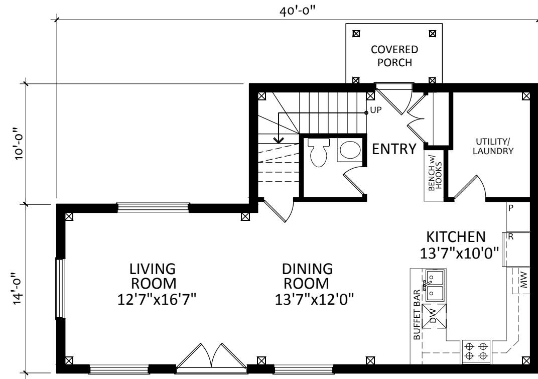
GROUND FLOOR PLAN 800 sq.ft.
