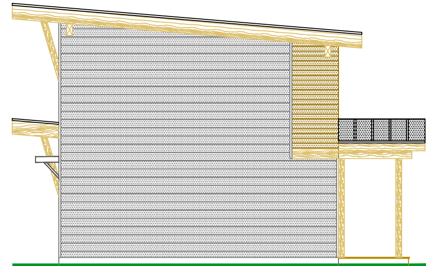
EAST ELEVATION
