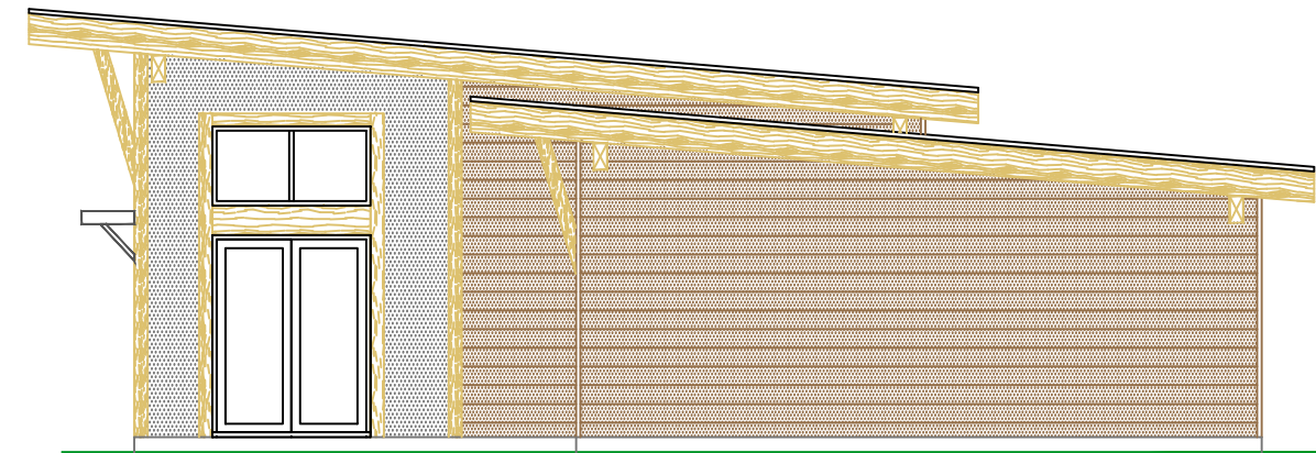
WEST ELEVATION
