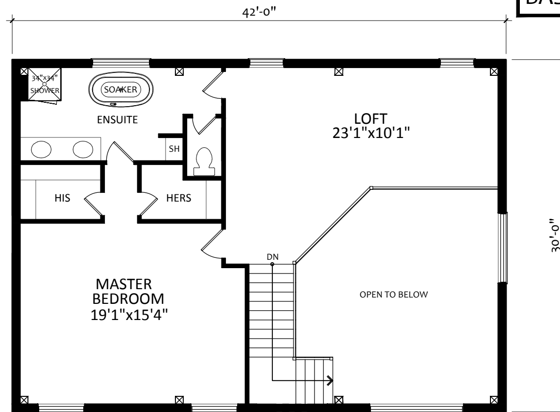
SECOND FLOOR PLAN 892 sq.ft.
