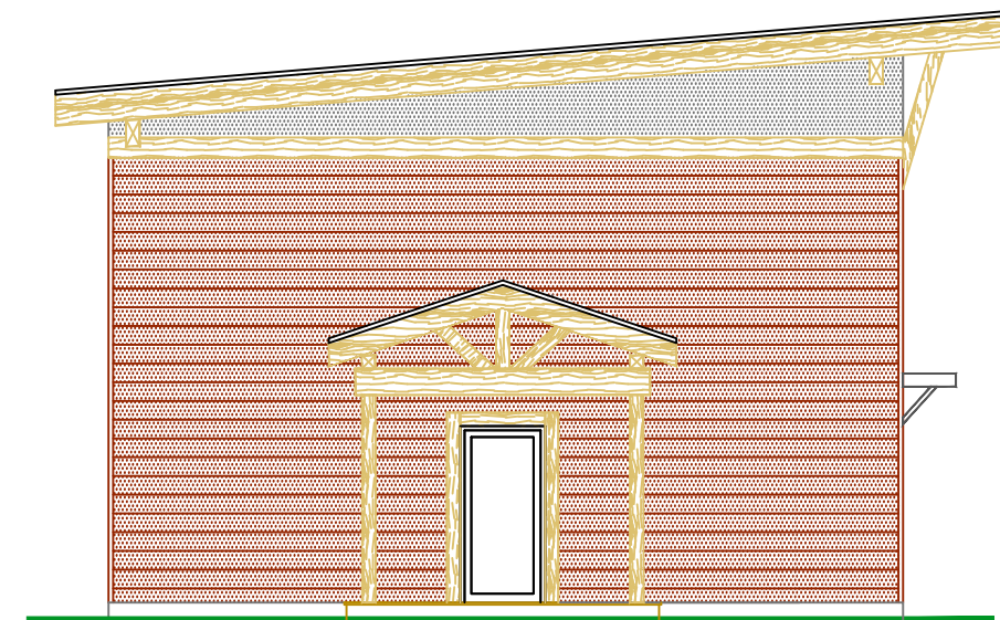
WEST ELEVATION
