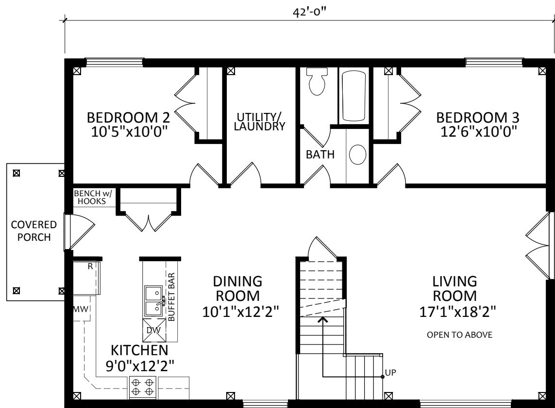
GROUND FLOOR PLAN 1260 sq.ft.
