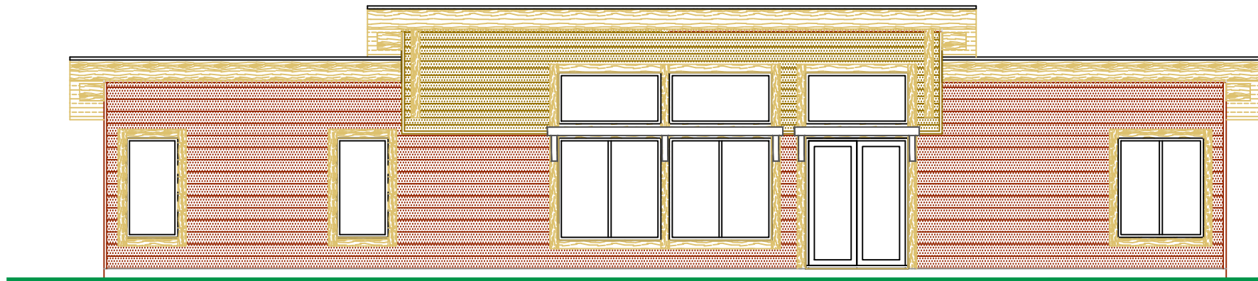
SOUTH ELEVATION
