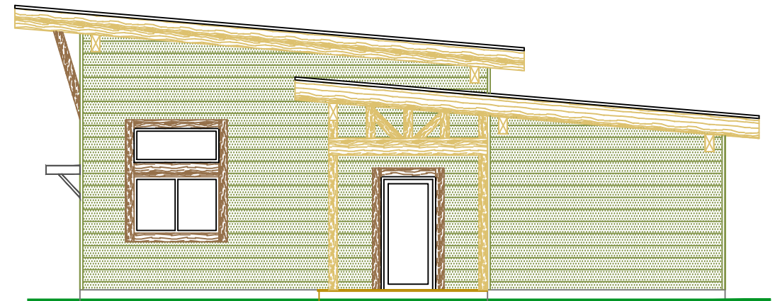
EAST ELEVATION
