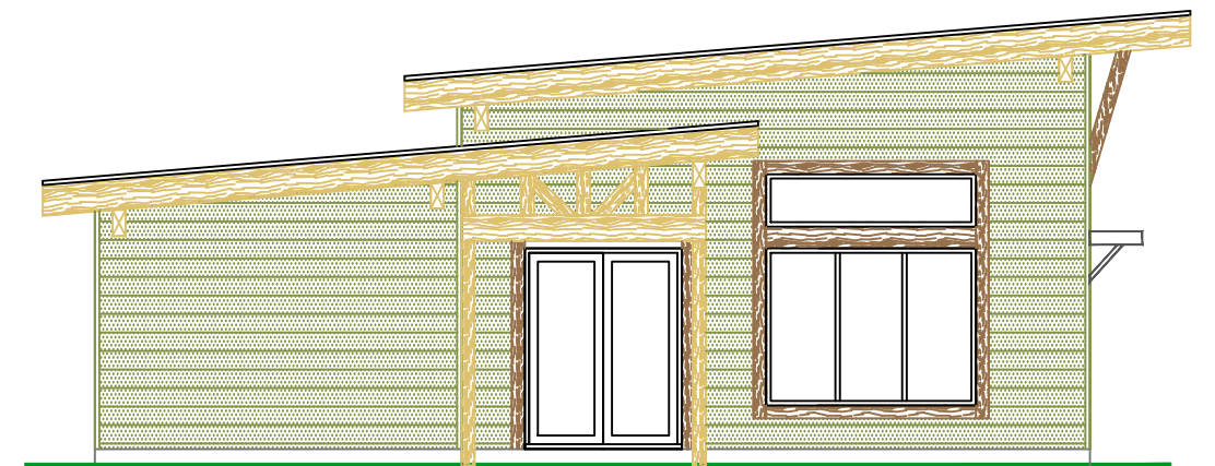
WEST ELEVATION
