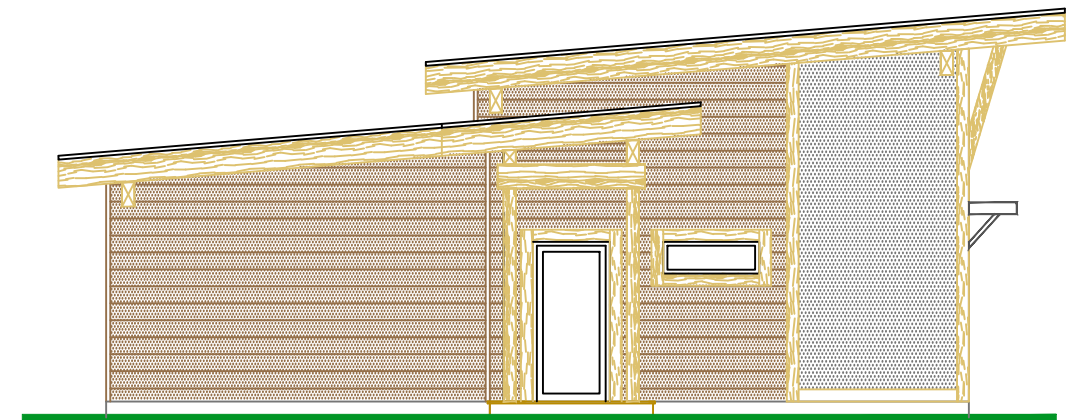
WEST ELEVATION
