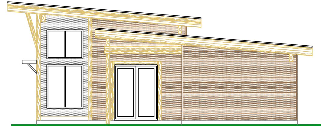
EAST ELEVATION
