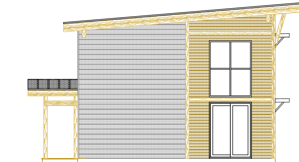
WEST ELEVATION
